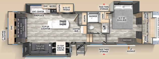
32LIVE LENGTH 36' 5" WIDTH 96" HEIGHT 13' 3" UVW 10,363 LB GVWR 13,500 LB HITCH 1,935 LB CCC 3,137 LB AWNING 15' & 11' FRESH 60 GAL GRAY 38 GAL BLACK 38 GAL
