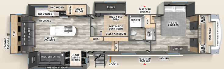
36MB LENGTH 42' 7" WIDTH 96" HEIGHT 13' 2" UVW 11,537 LB GVWR 14,335 LB HITCH 2,335 LB CCC 2,798 LB AWNING 19' & 11' FRESH 60 GAL GRAY 76 GAL BLACK 38 GAL
