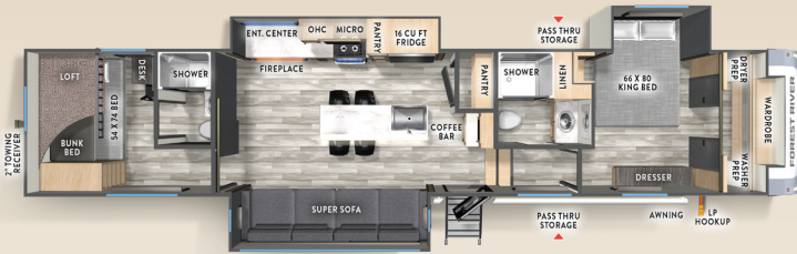
35CRIB LENGTH 42' 8" WIDTH 96" HEIGHT 13' 6" UVW 11,953 LB GVWR 14,305 LB HITCH 2,305 LB CCC 2,352 LB AWNING 10' 6" & 14' FRESH 60 GAL GRAY 76 GAL BLACK 76 GAL
