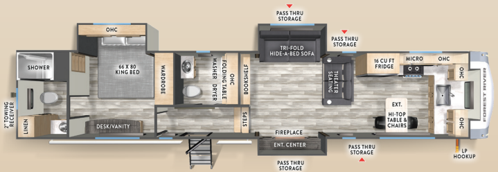
37GALLEY LENGTH 42' 9" WIDTH 96" HEIGHT 13' 5" UVW 11,123 LB GVWR 14,080 LB HITCH 2,080 LB CCC 2,957 LB AWNING 19' FRESH 60 GAL GRAY 76 GAL BLACK 76 GAL
