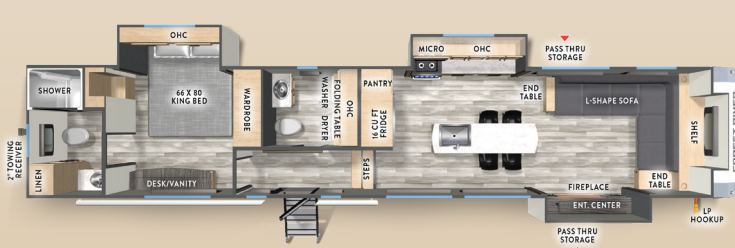
37PUB LENGTH 42' 9" WIDTH 96" HEIGHT 13' 5" UVW 10,873 LB GVWR 14,050 LB HITCH 2,050 LB CCC 3,177 LB AWNING 19' FRESH 60 GAL GRAY 76 GAL BLACK 76 GAL
